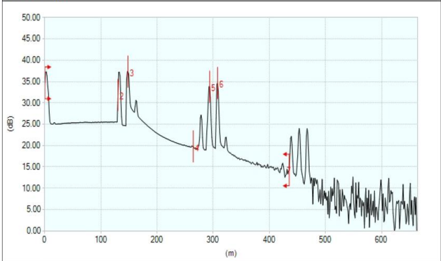
Optical time-domain reflectometer
